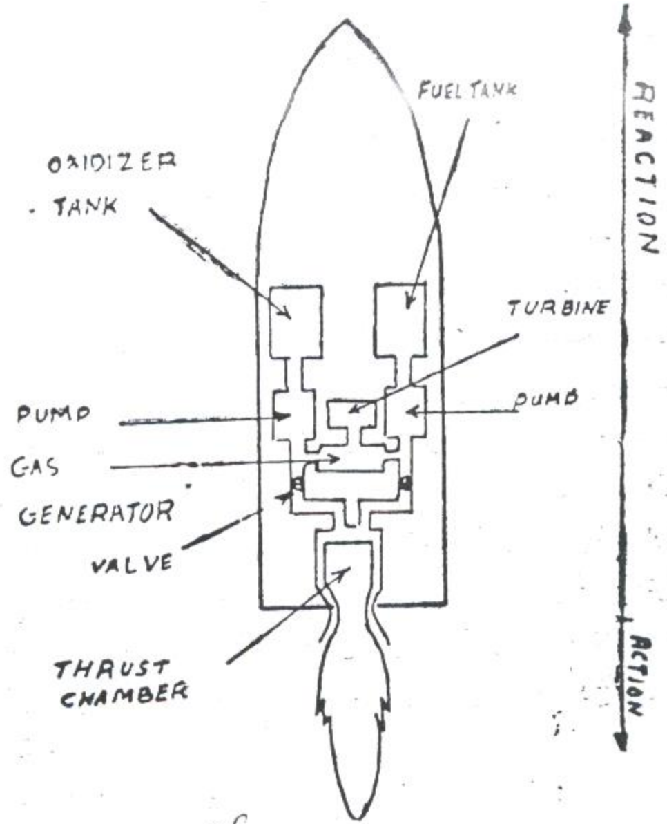
Diagram of liquid-fueled rocket.
